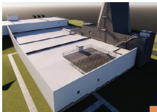
Hangarettes concept drawing
