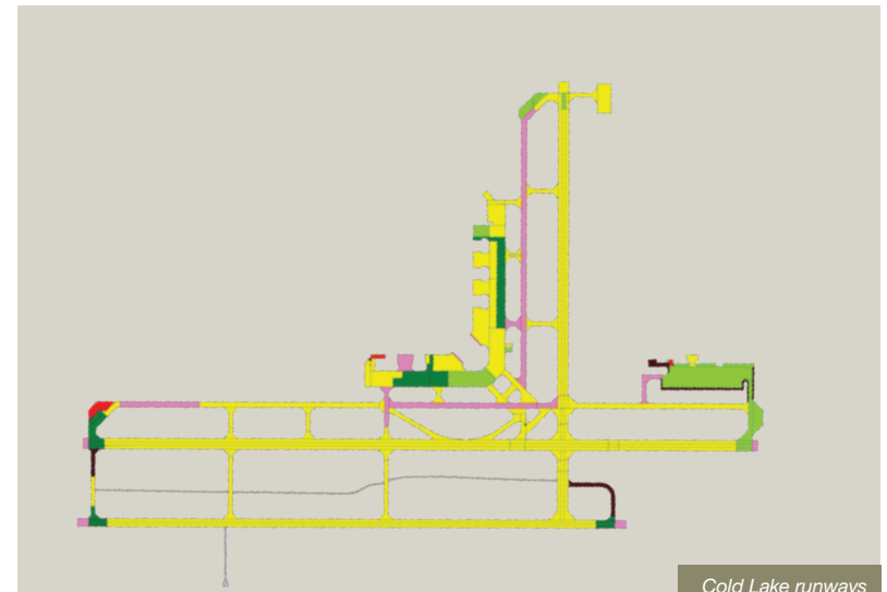
Cold Lake runways
