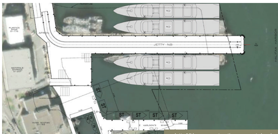
Jetty NH new construction concept drawing
